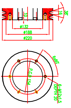
CRANK SHAFT PULLEY(S=2/1)
