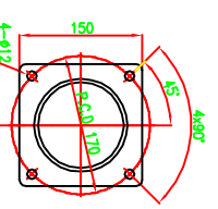
EXHAUST ELBOW FLANGE(2/1)
